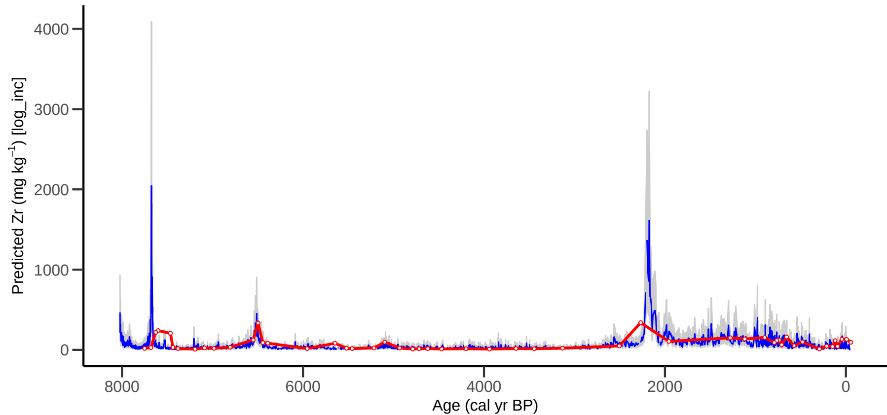
KER1: PLSR Zr Predictions with Confidence Interval (log_inc model)
